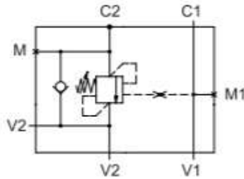
Typical Single Counterbalance Parts-in-body.
