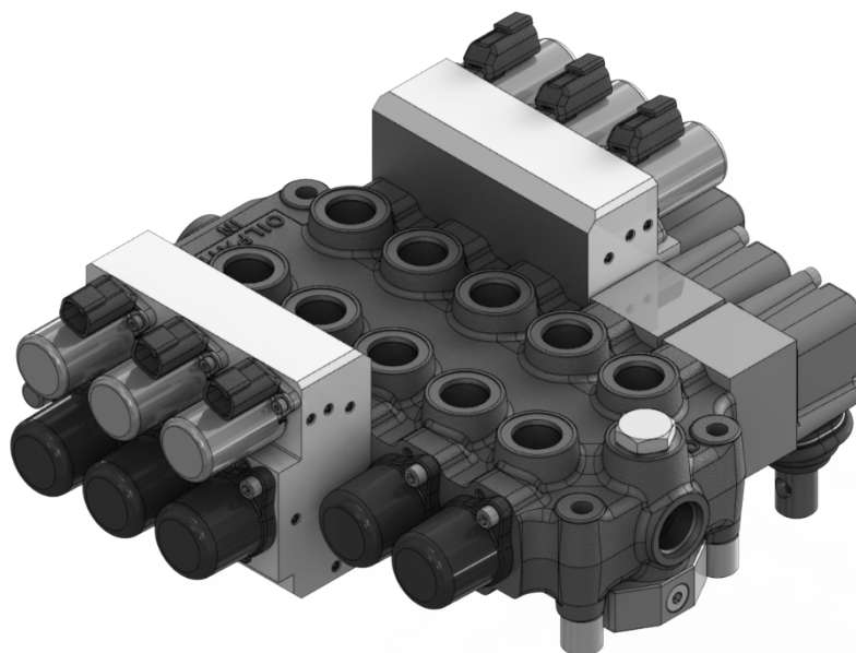
OP20 configured with 3 solenoid actuated spools with manual override and 2 manually operated spools (in the upside-down configuration). Typically utilised in Tilt Tray applications
